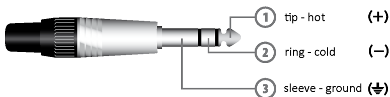
Jack (balanced)
